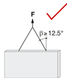
Traction oblique
