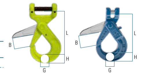
Crochet sangle BKWX
